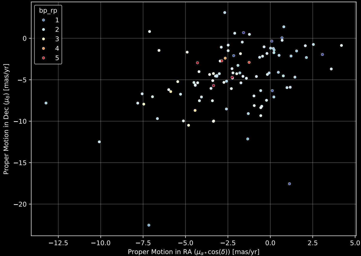
APOGEE DR17 Field: [009+09] Proper Motion Diagram (n= 107)
