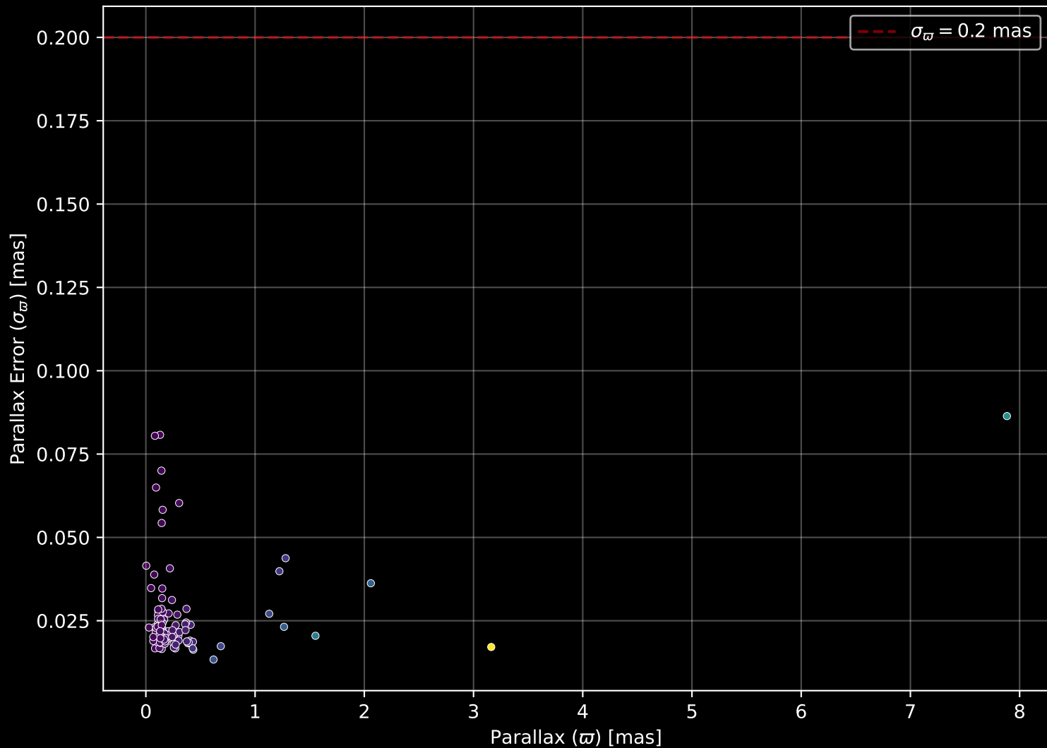
APOGEE DR17 Field: [009+09] Parallax Quality (n= 107)
