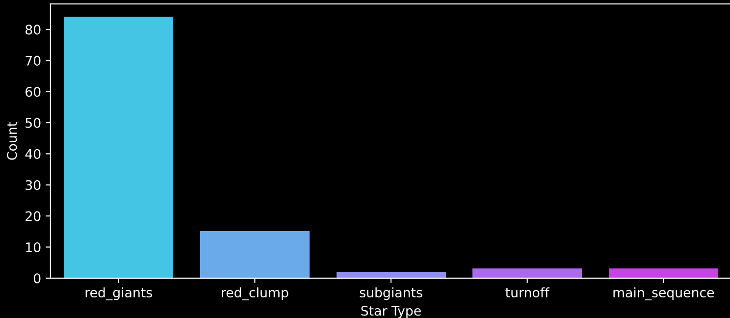
APOGEE DR17 Field: [009+09] Count plot of Star Type
