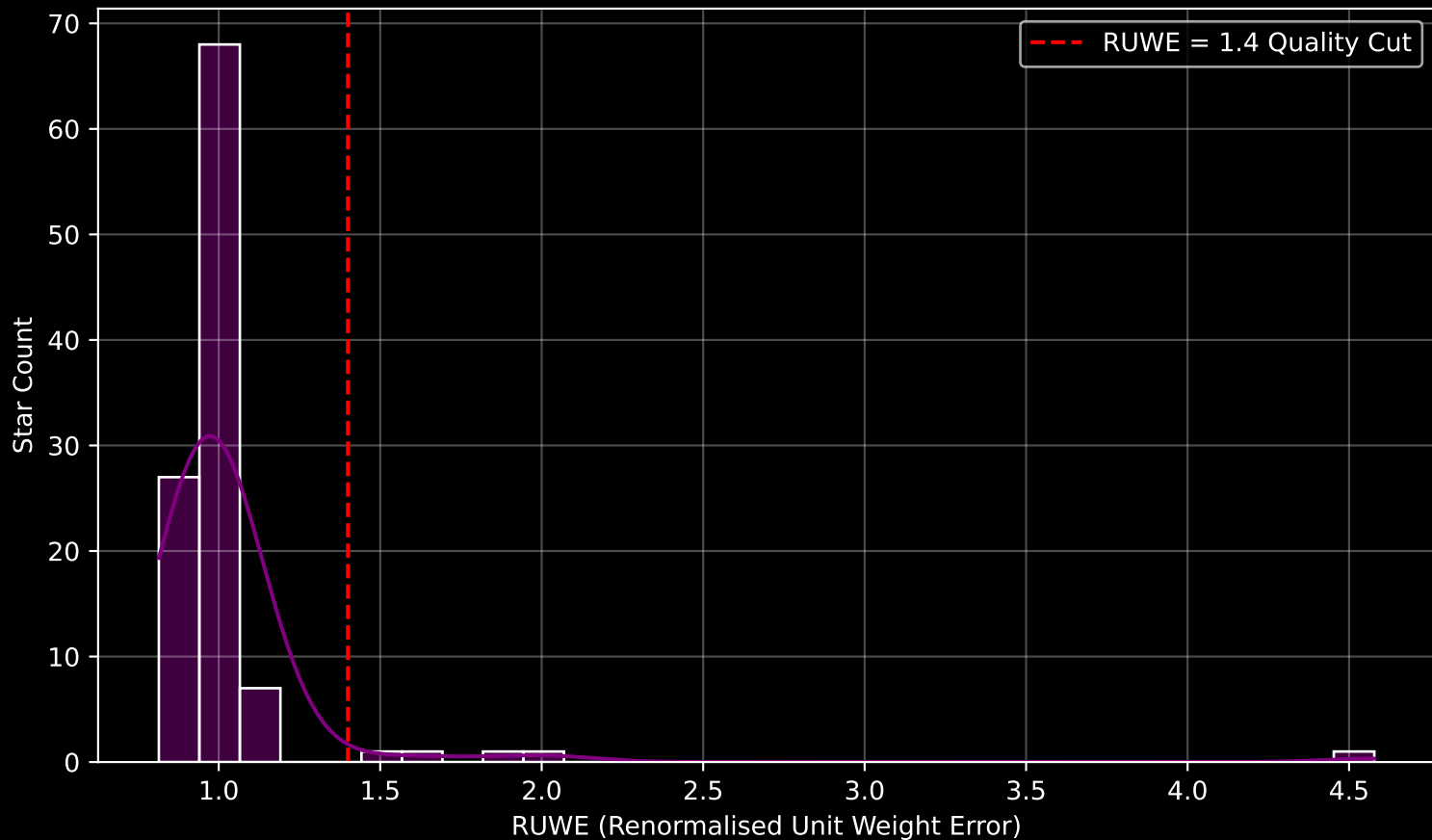
GAPOGEE DR17 Field [009+09] RUWE Distribution (n= 107)
