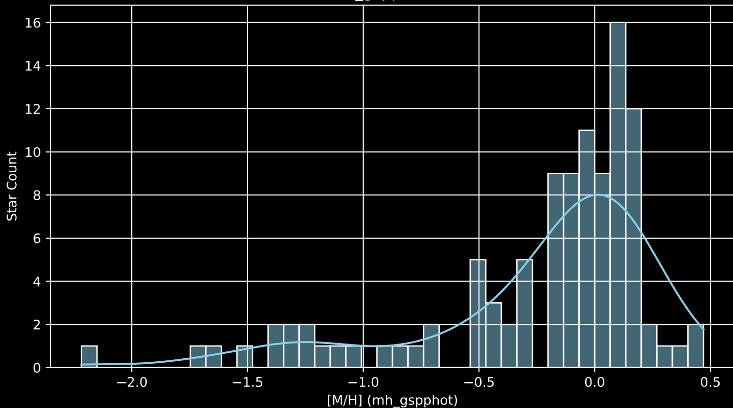
APOGEE DR17 Field: [009+09 [M/H] (mh_gspphot) (n= 105)
