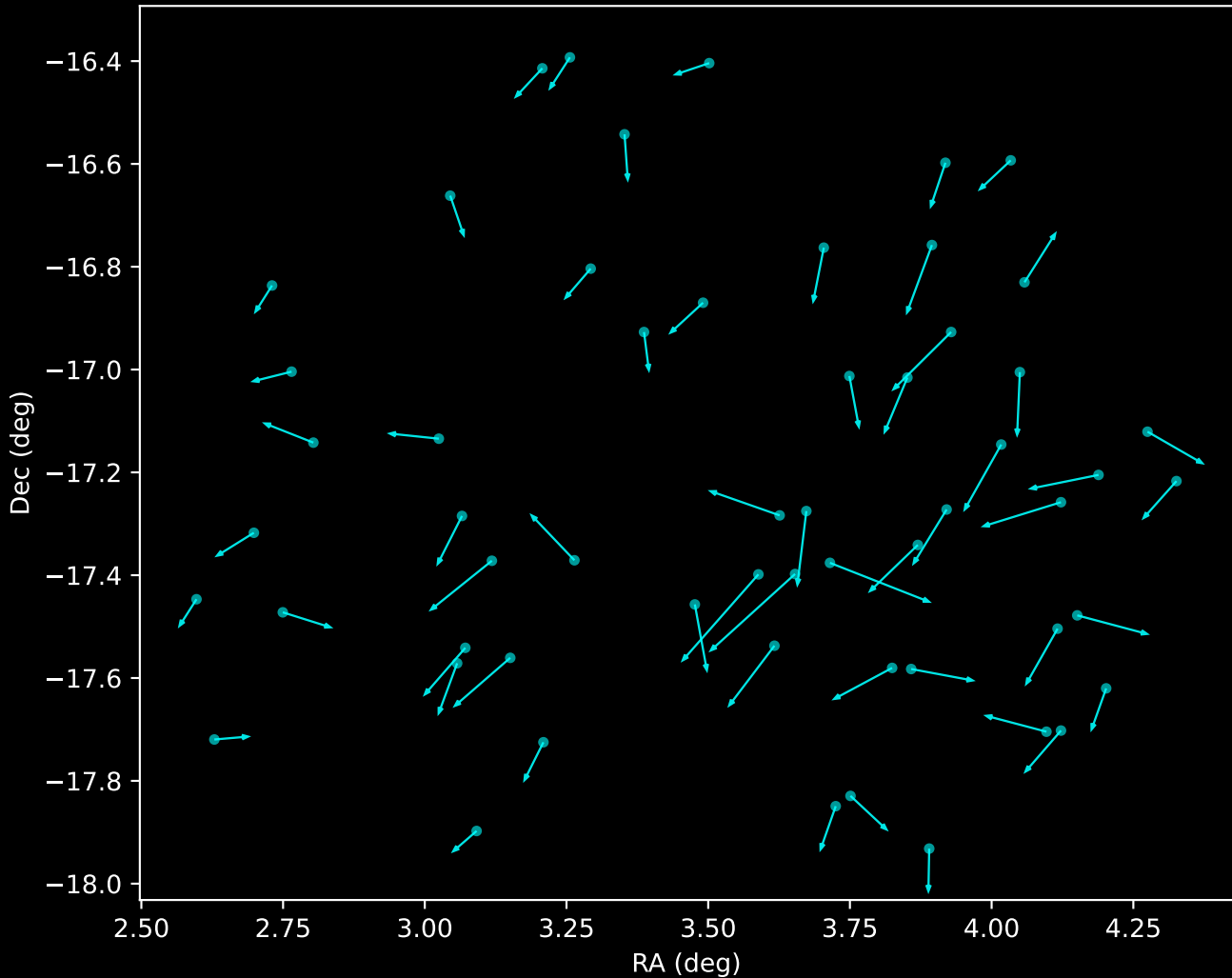
APOGEE DR17 Noise Stream Proper Motion Vectors (n=57)
