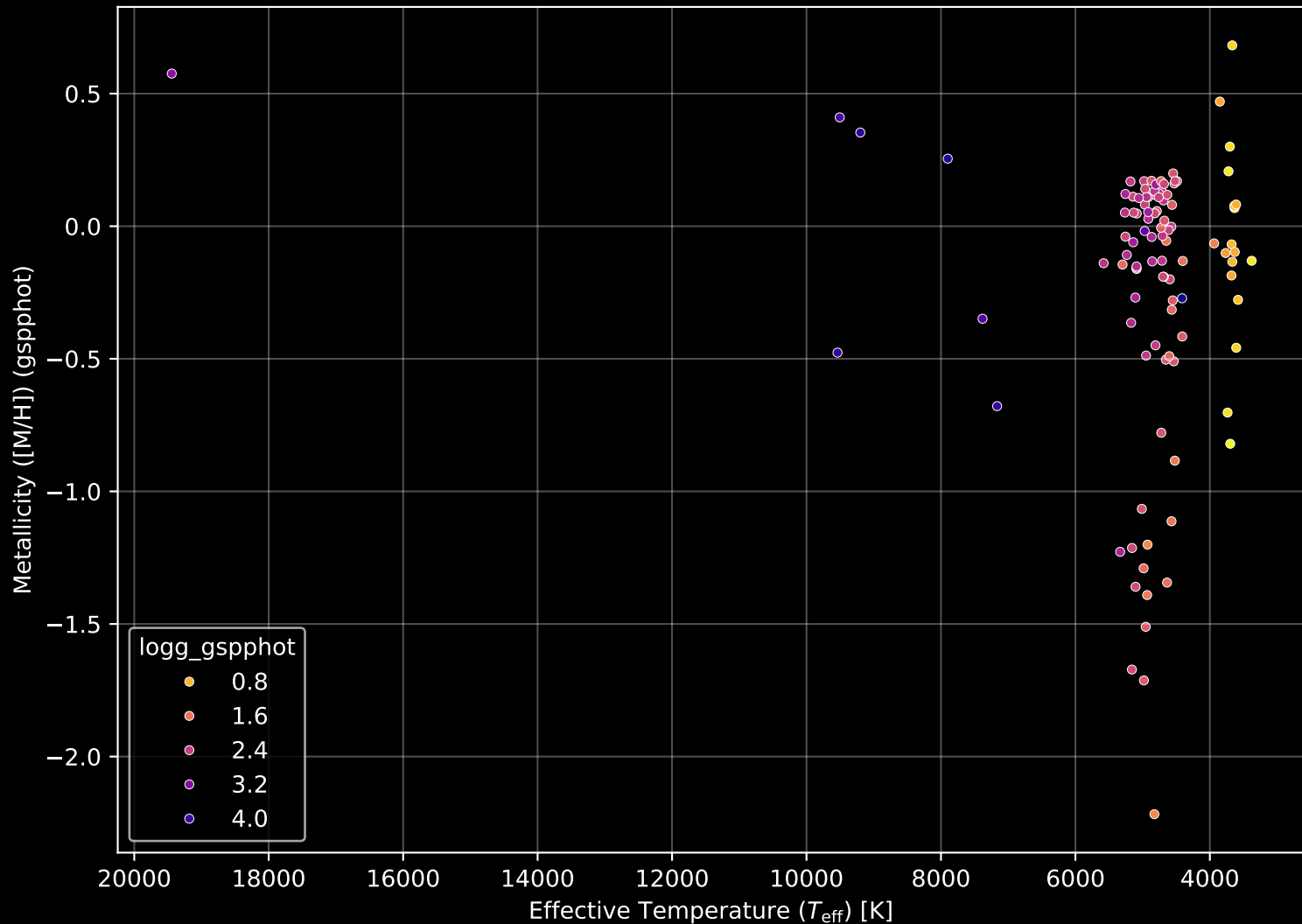
APOGEE DR17 Field: [009+09] Stellar Population Parameters (n= 107)
